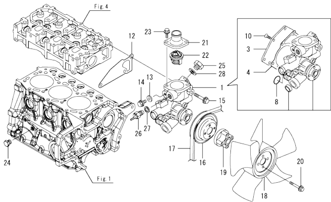
Fig.9. COOLING WATER SYSTEM
