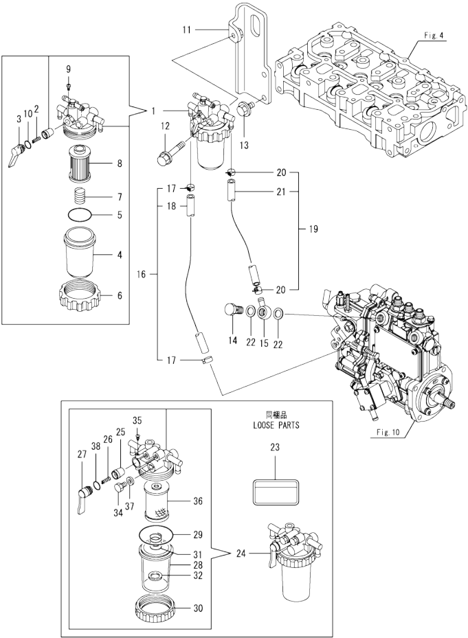
Fig.13. FUEL LINE
